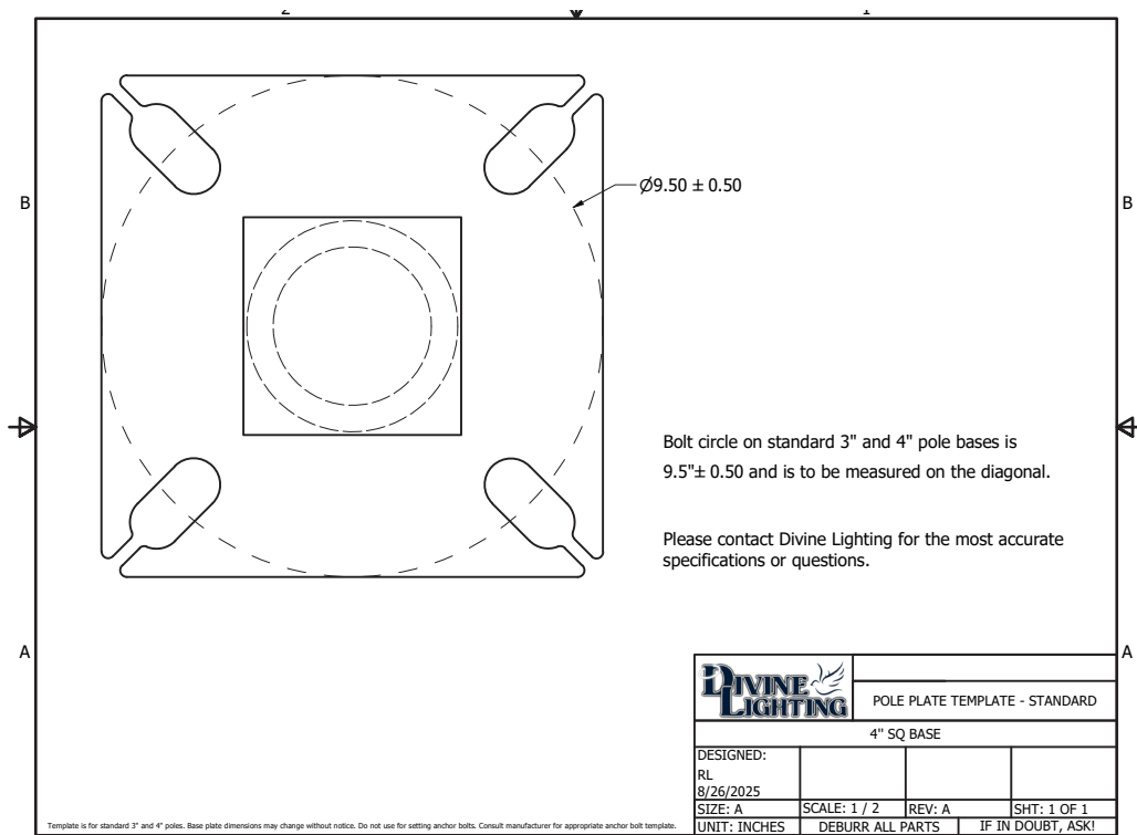
3" & 4" Pole Template
