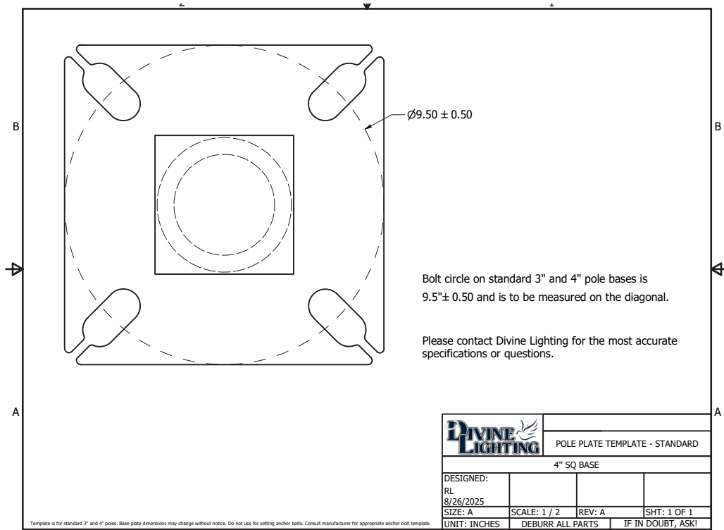
3" & 4" Pole Template
