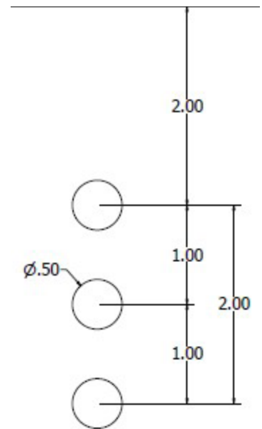
Divine Standard Drill Pattern
