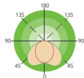
Textured Diffuser (Aisle Optic)
