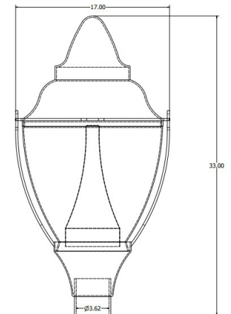
Pattern 1B & 2B Dimensions
