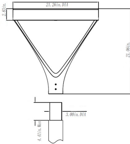
Post Top EPA: 0.64 Sq. Ft. Weight: 29.76 lbs.
